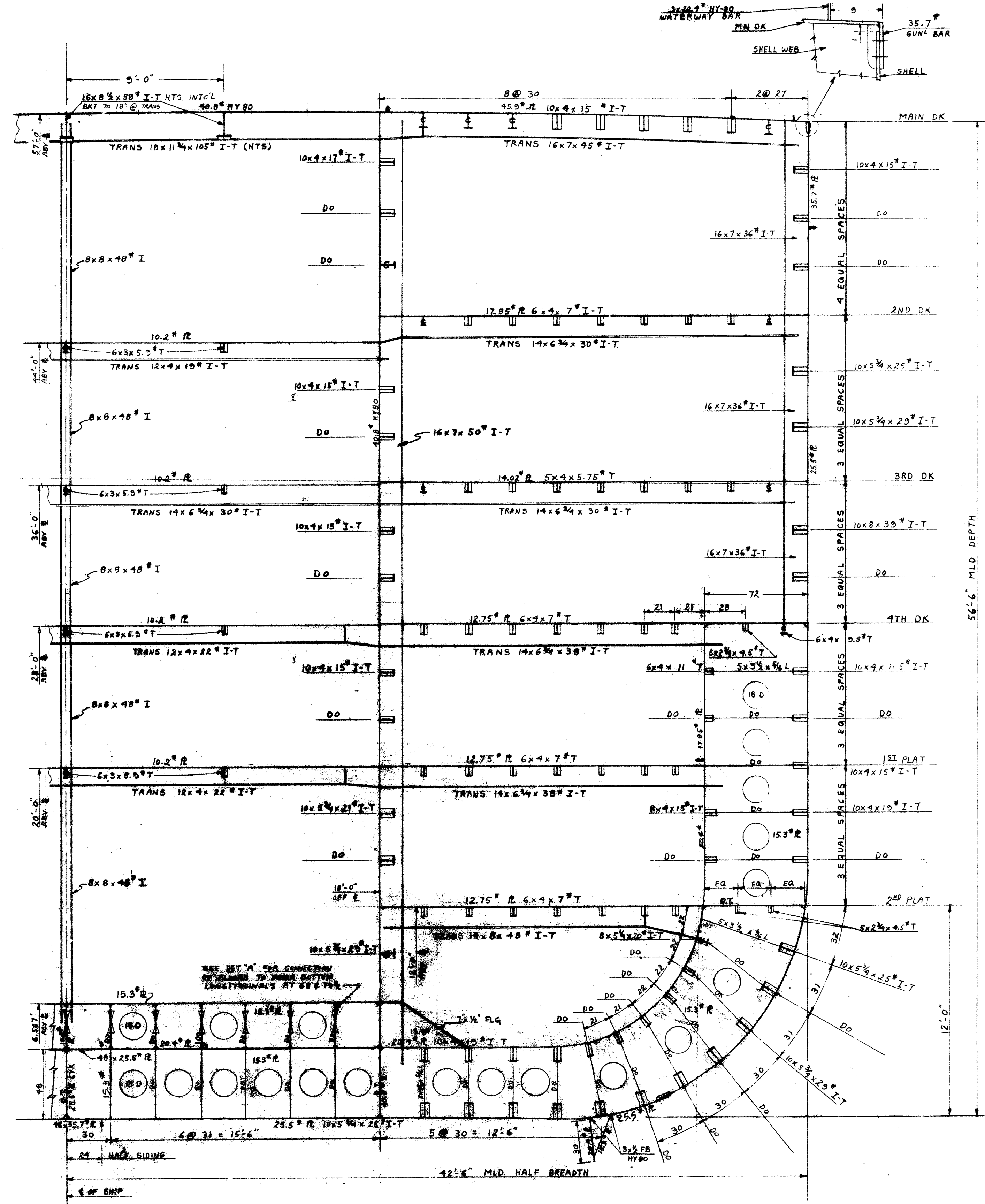
MIDSHIP SECTION
