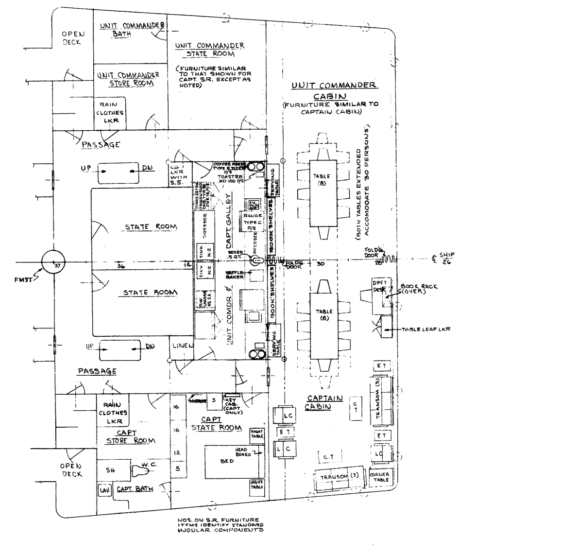
O3 LEVEL UNIT COMDR & CAPTAIN QUARTERS SCALE 1/4"=1'-0"
