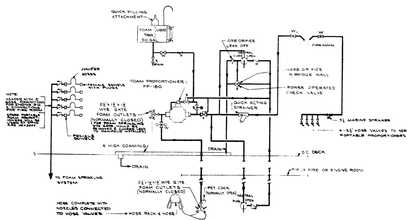
DIAGRAMMATIC ARRANGEMENT OF FOAM STATION DETAIL A
