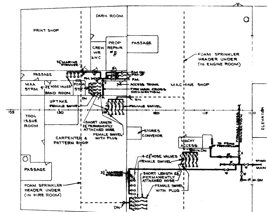
DIAGRAMMATIC ARRANGEMENT OF FOAM STANDPIPES 2ND DECK DETAIL B
