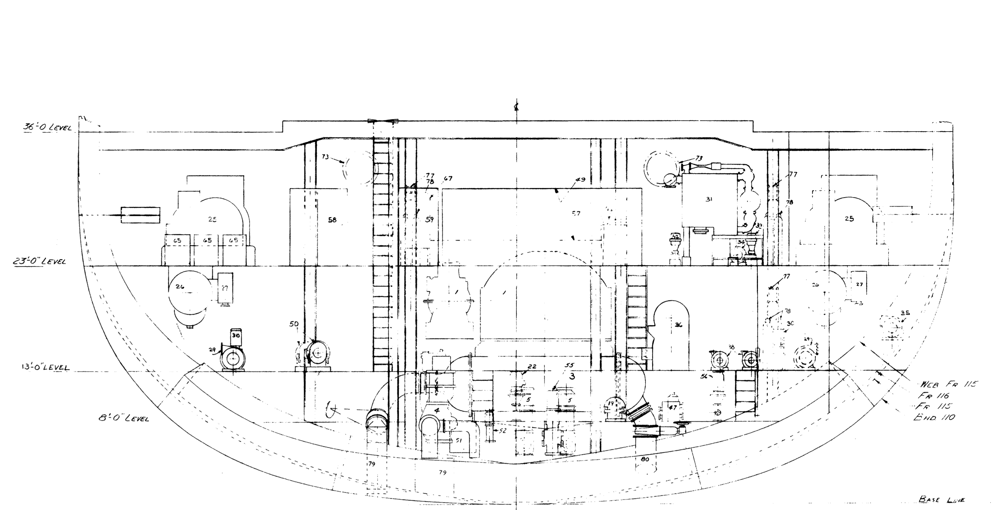
SECTION AT BHD 110 LOOKING AFT.
