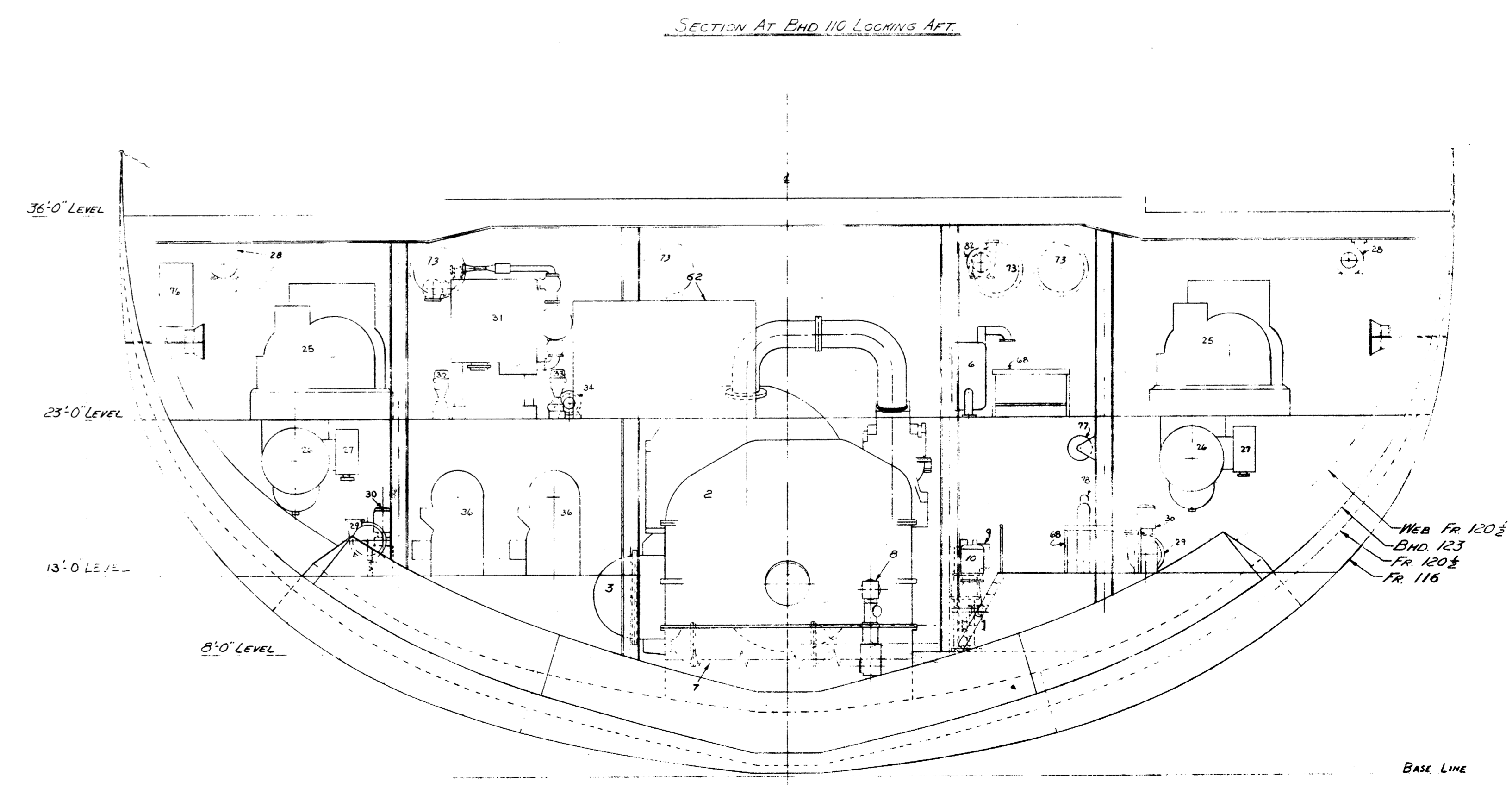
SECTION AT BHD 123 LOOKING FWD.
