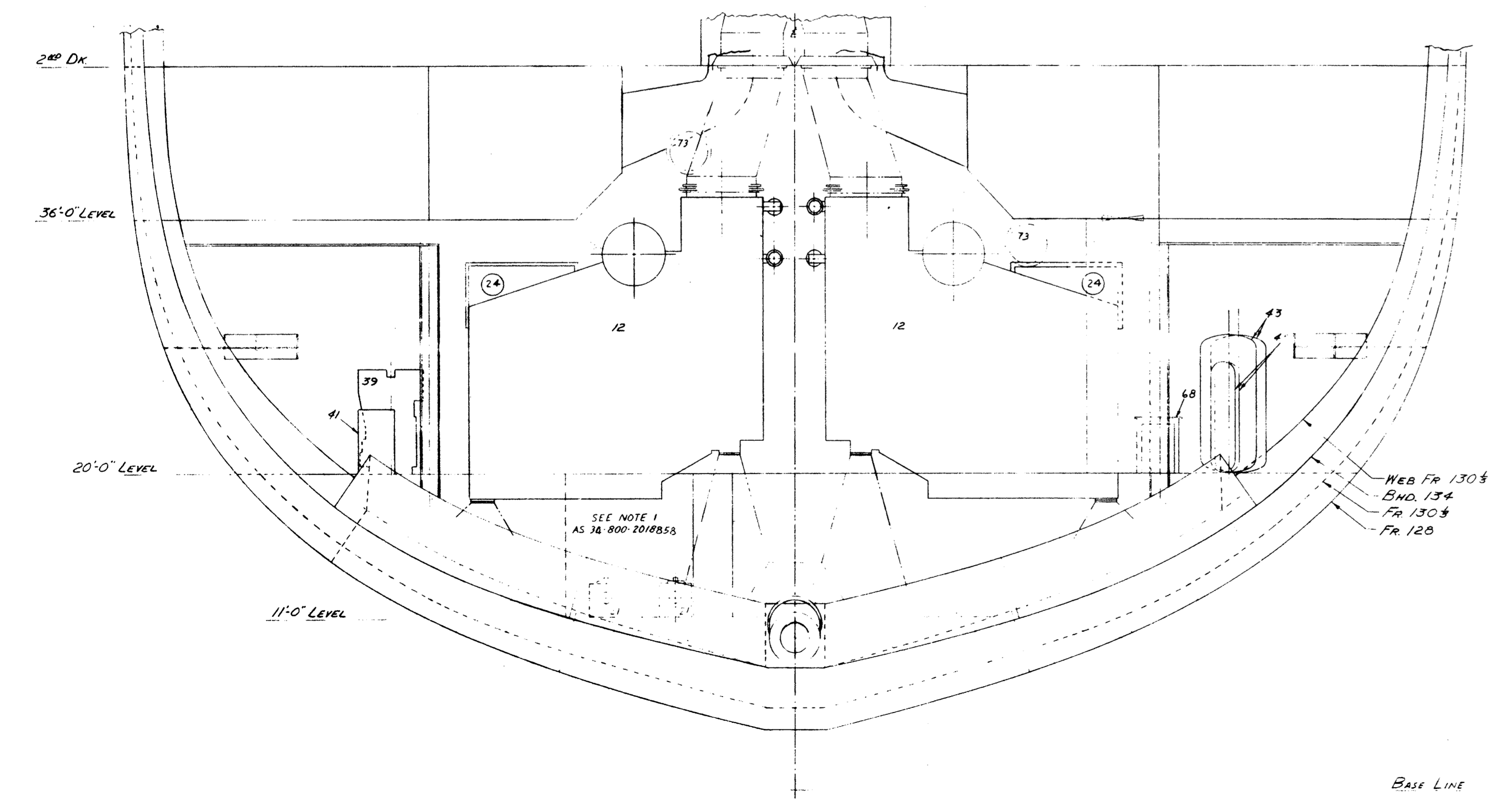
SECTION AT BHD 134 LOOKING FWD.
