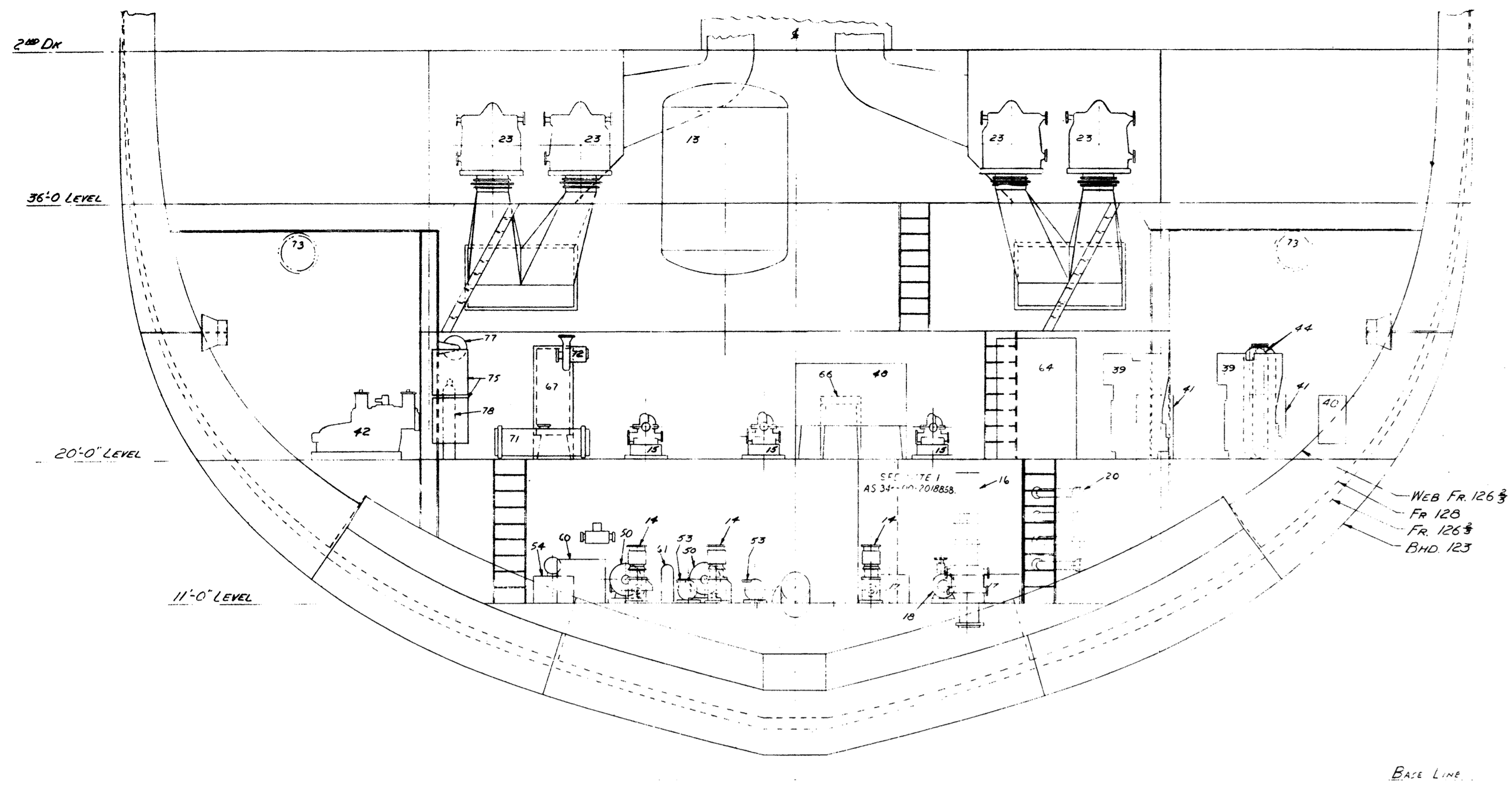
SECTION AT BHD 123 LOOKING AFT.
