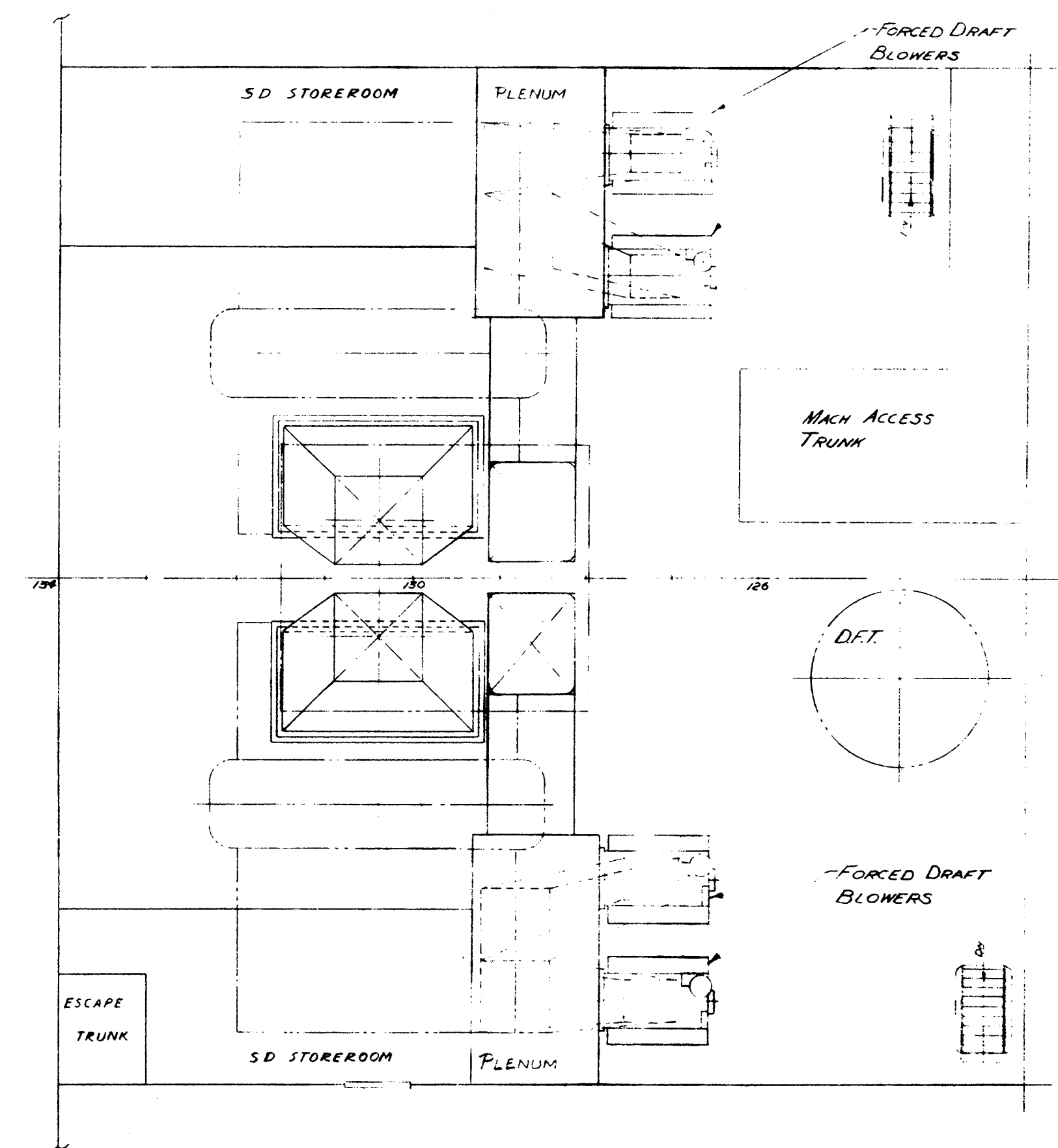
PLAN - THIRD DECK
