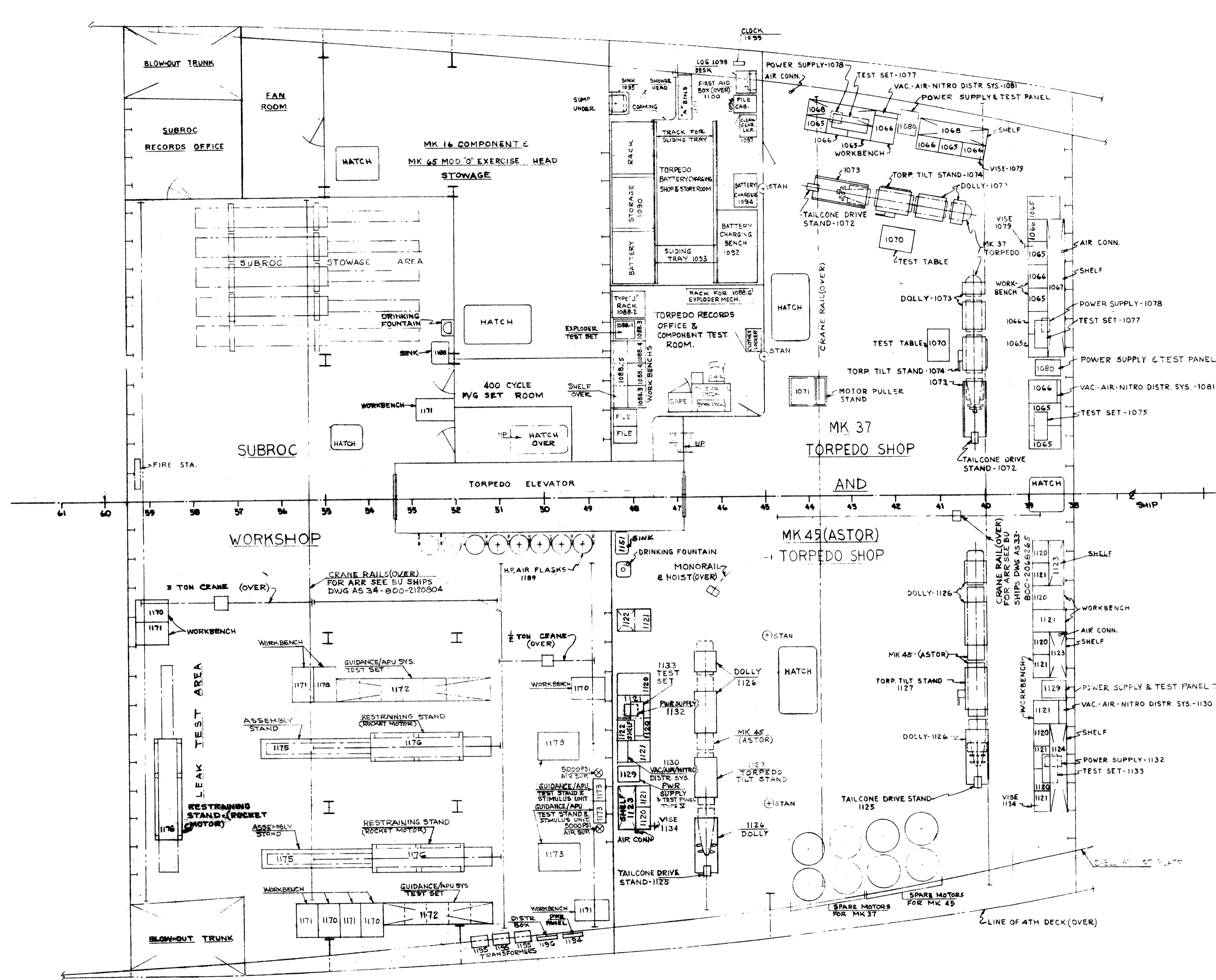
PLAN - 1ST PLATFORM
