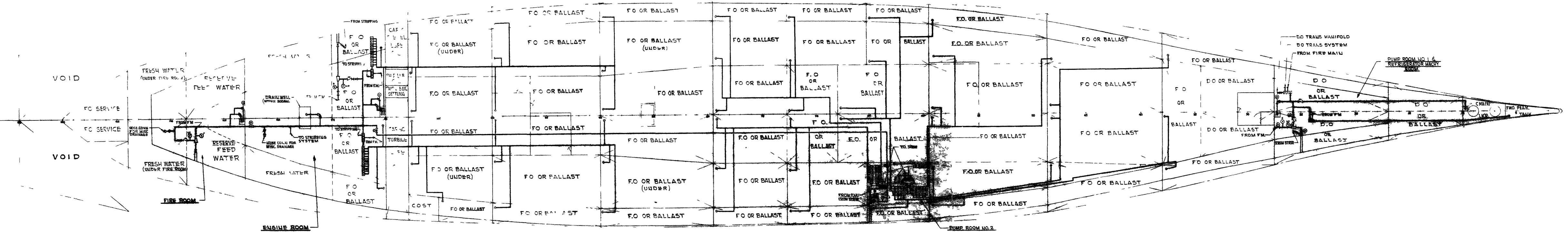
DRAINAGE AND BALLAST SYSTEM
