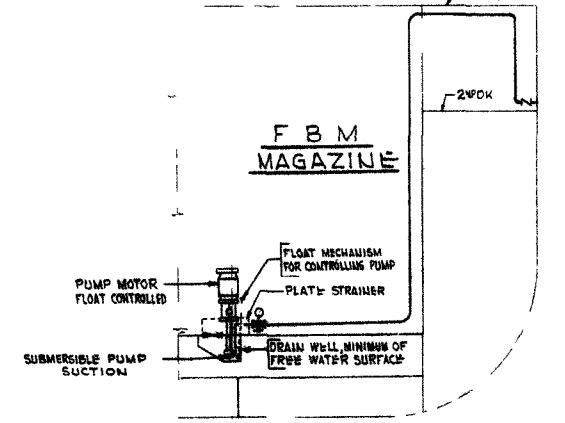
SECTION AT FR 79 1/2 LKG FWD NOT TO SCALE
